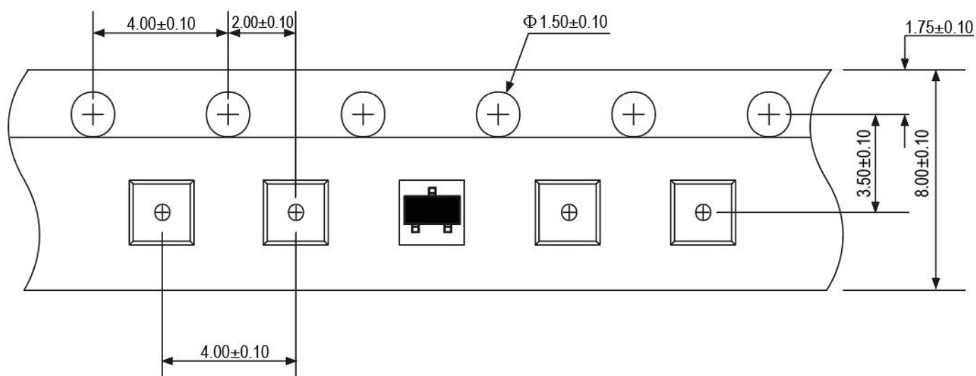
Tape Dimensions
