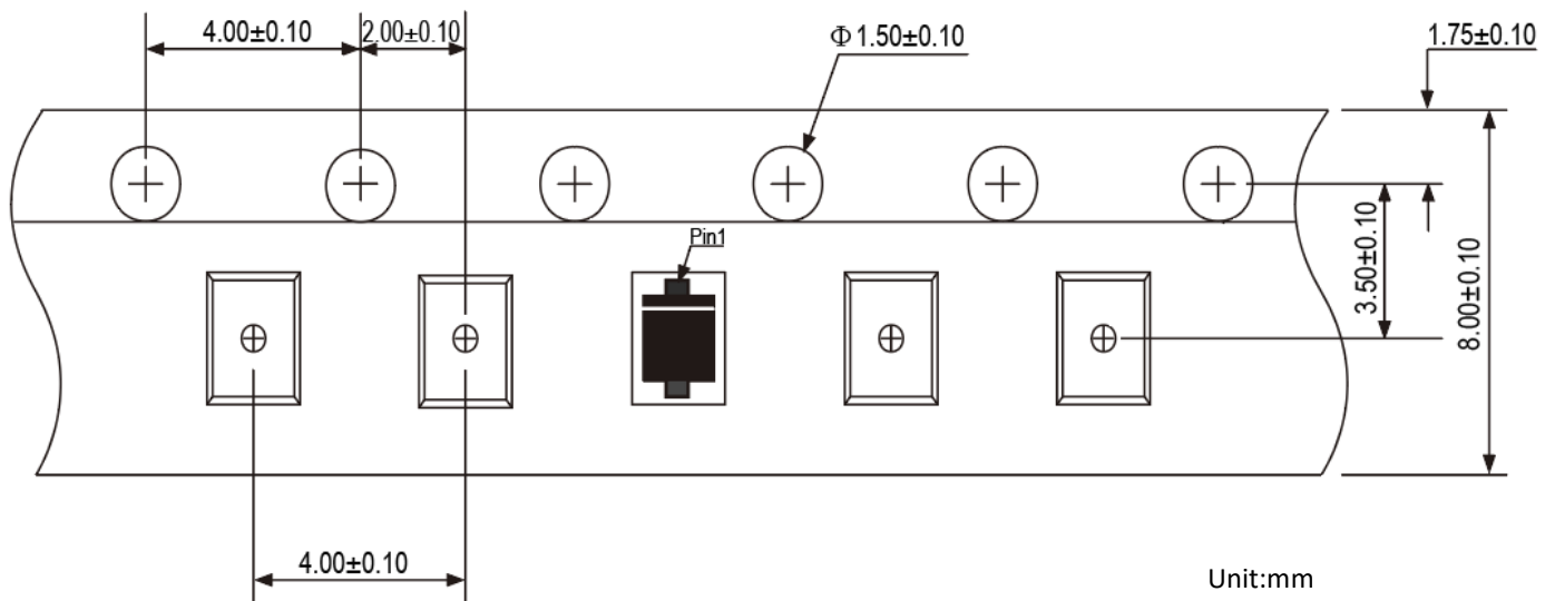
Tape Dimensions
