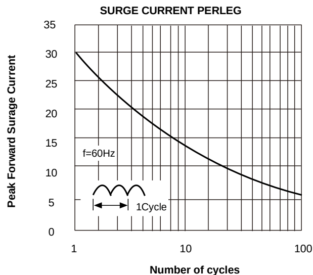
FIG.2-MAXIMUM NON-REPETITIVE PEAK FORWARD
