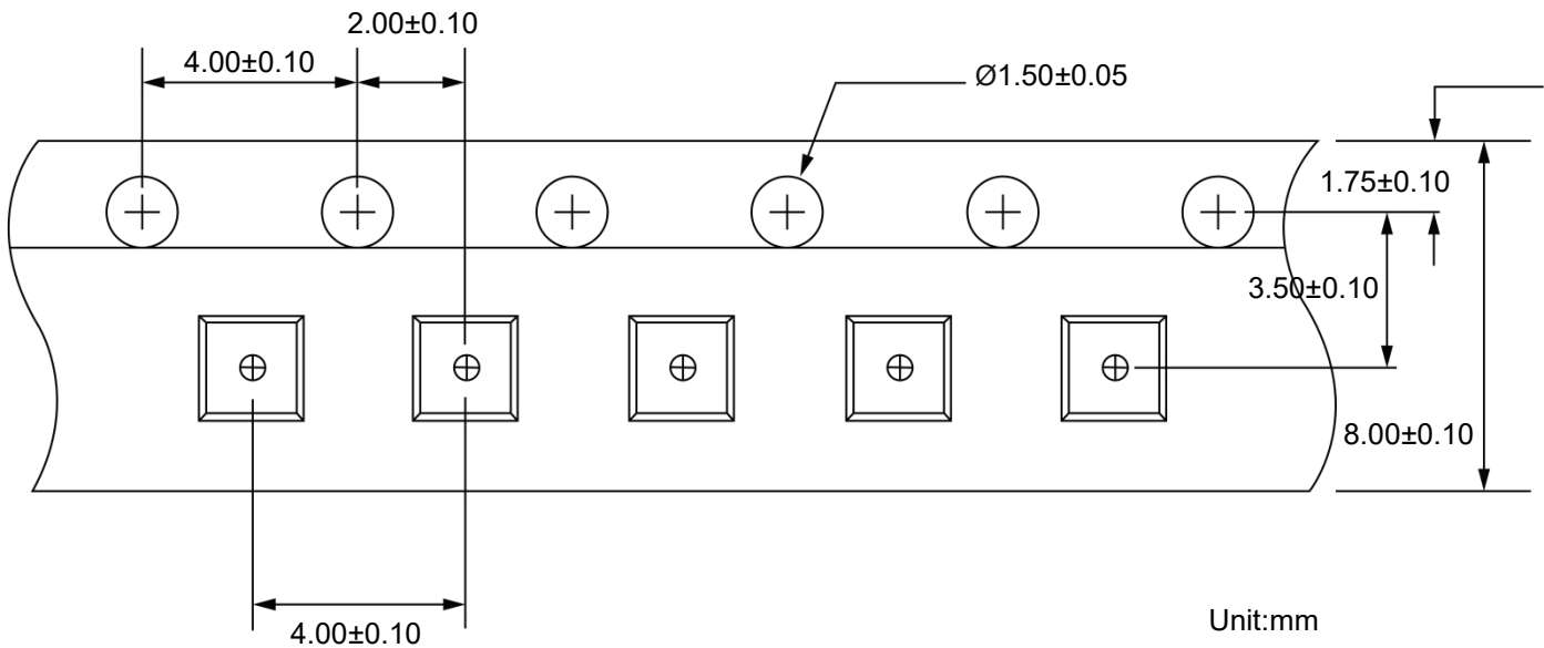
Tape Dimensions
