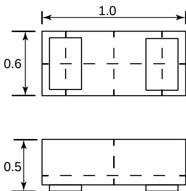
Package Dimensions
