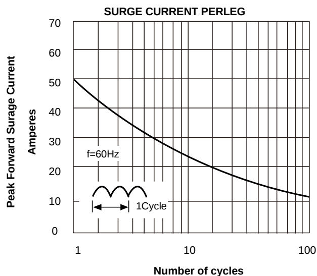
FIG.2-MAXIMUM NON-REPETITIVE PEAK FORWARD
