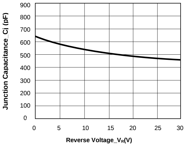
Junction Capacitance vs. Reverse Vlotage
