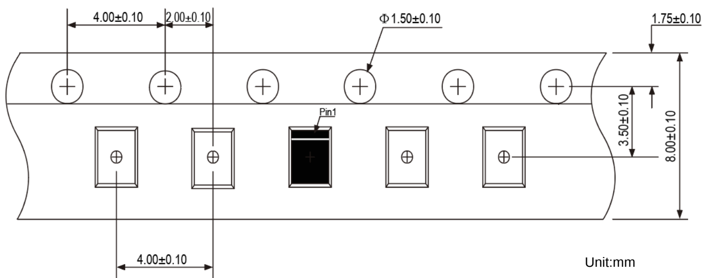
Tape Dimensions
