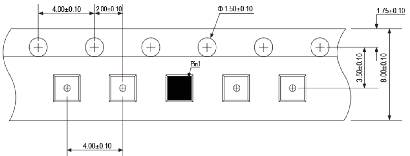
Tape Dimensions
