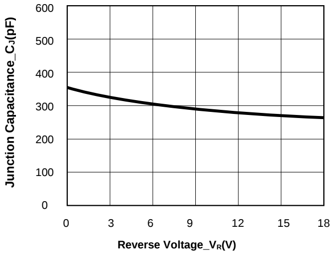
Junction Capacitance vs. Reverse Vlotage
