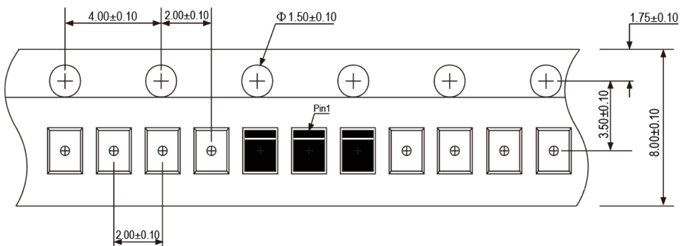
Tape Dimensions
