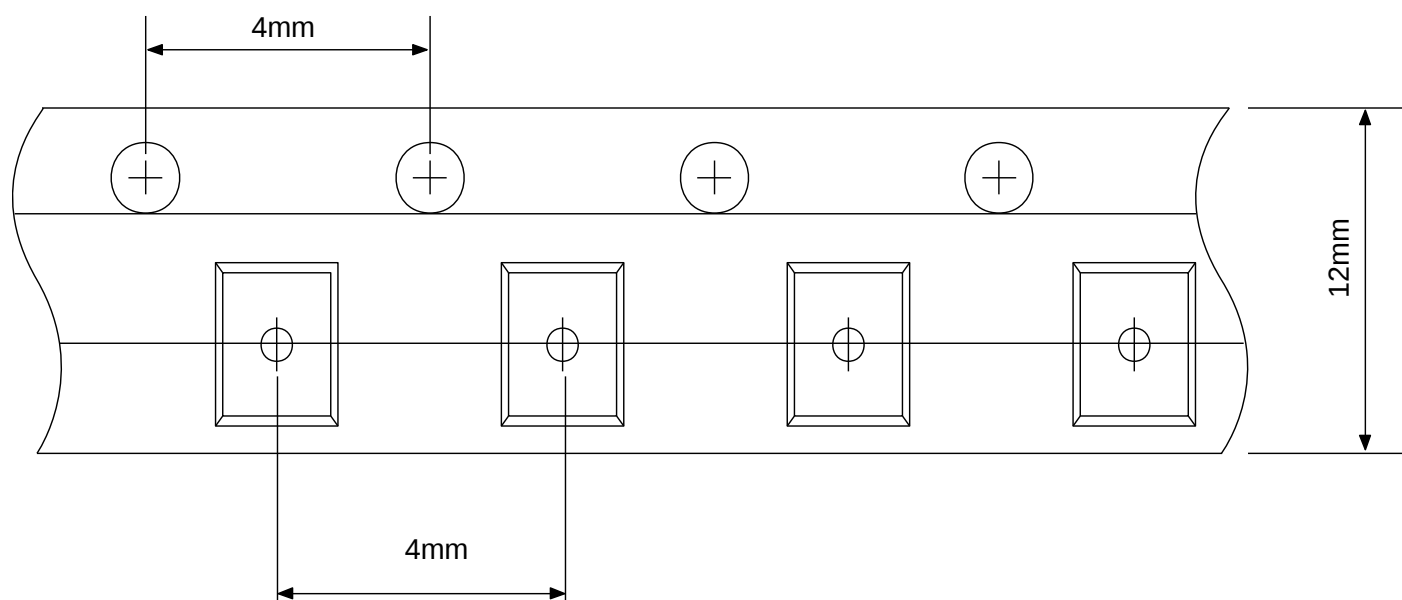
Tape Dimensions
