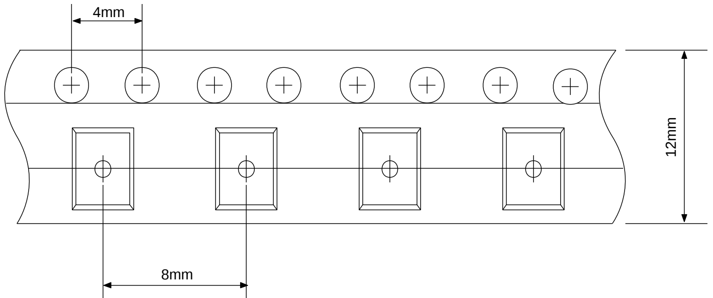
Tape Dimensions
