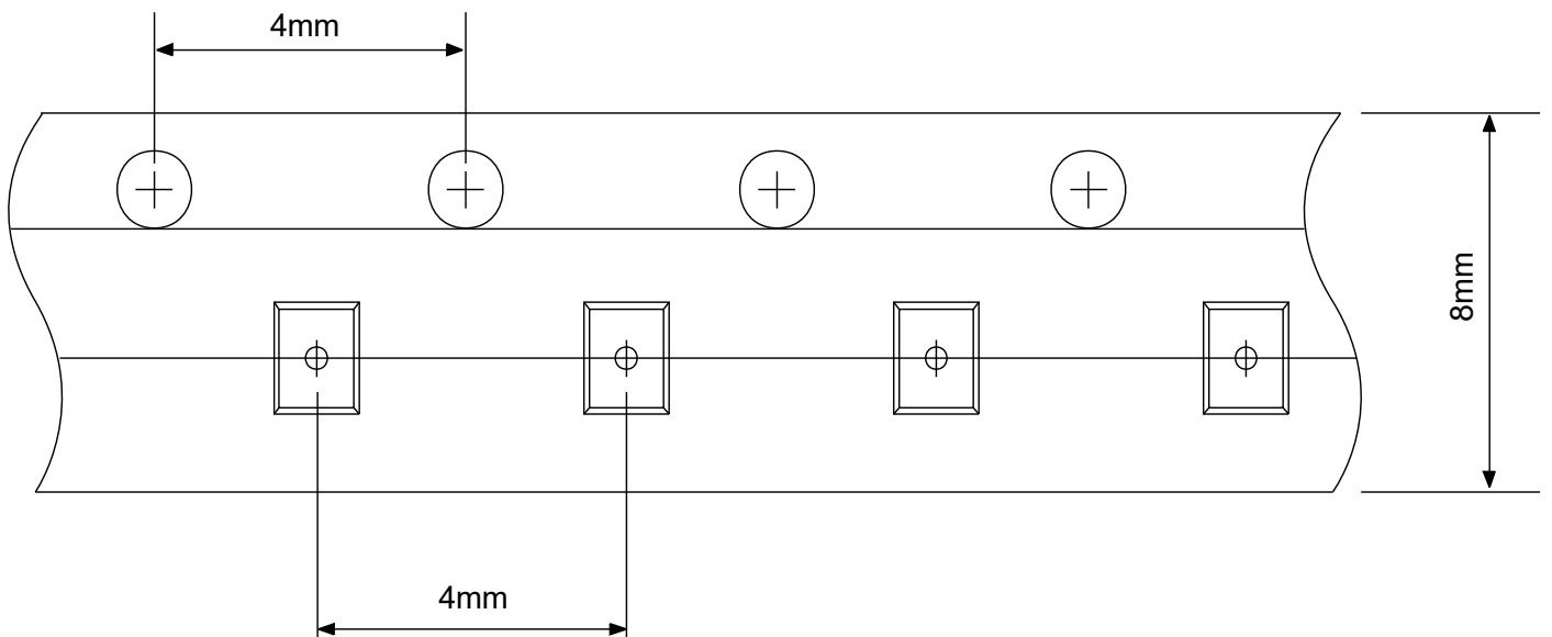
Tape Dimensions
