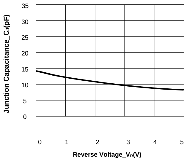
Junction Capacitance vs. Reverse Vlotage
