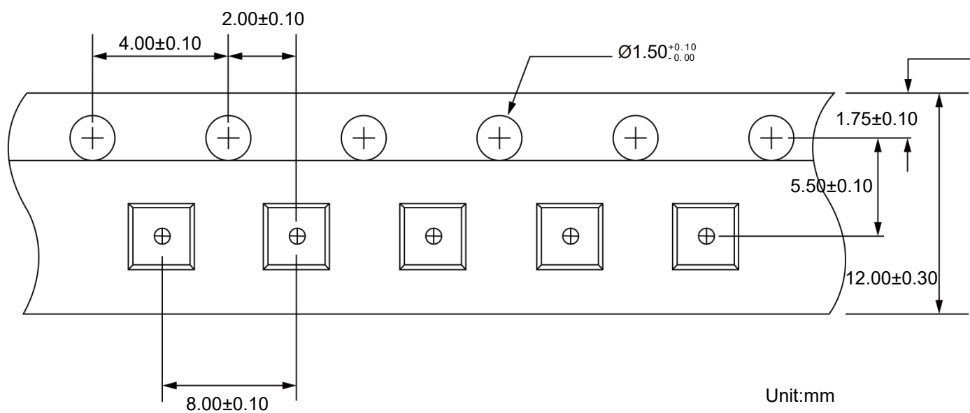
Tape Dimensions
