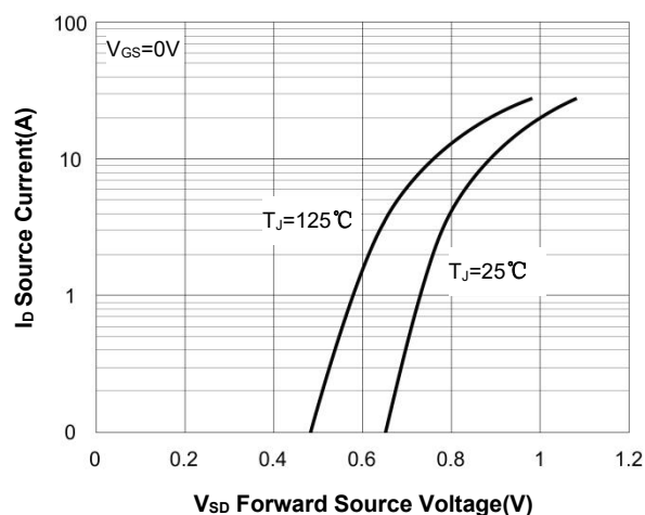
Source Current vs. Forward Source Voltage
