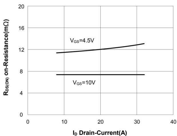
R_{DS(ON)} On-Resistance vs. Drain-Current
