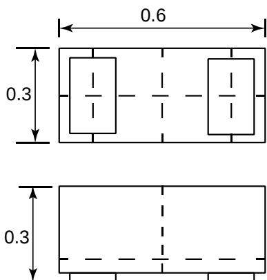
Package Dimensions
