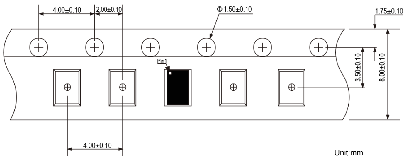
Tape Dimensions
