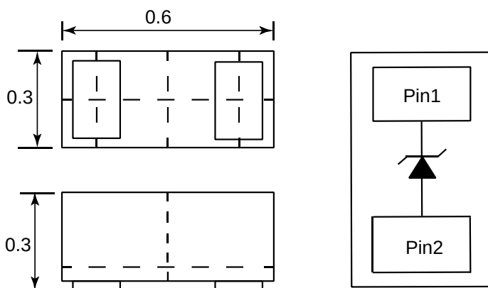
Package Dimensions
