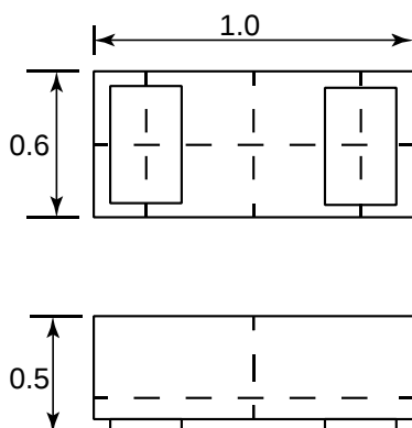
Package Dimensions
