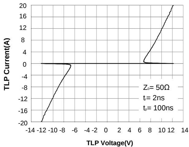
TLP Measurement
