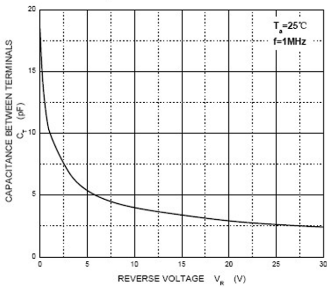
Capacitance Characteristics
